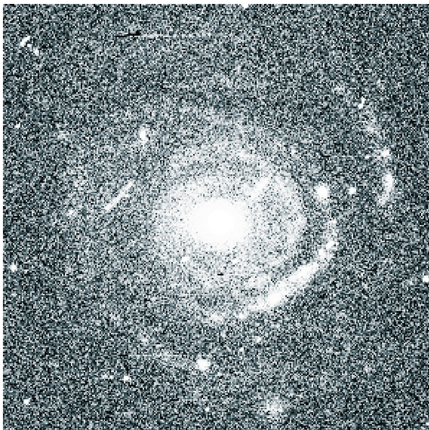
MALINIZATION TECHNIQUE enables the imaging of low-surface-brightness galaxies. This one is known, appropriately enough, as Malin 2; it was discovered in 1990 and was the second such galaxy to be found. It is about 450 million light-years away and, with a scale length of 15 kiloparsecs, is about five times the size of the Milky Way.
