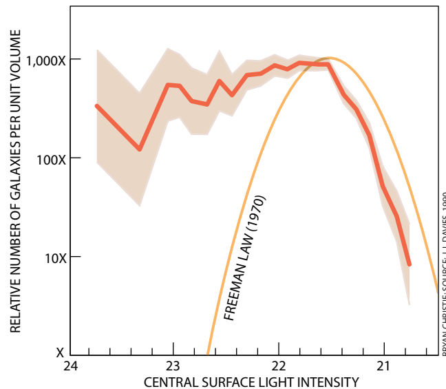
CHART OF RELATIVE SPACE DENSITY of galaxies shows that there are probably as many very diffuse galaxies, with central surface light intensities of 23 or 24 apparent magnitudes per square arc second, as there are conventional galaxies for which this value is about 21.5 or 22. (The shading indicates the range of uncertainty in the values.) The orange arc indicates how galaxies were thought to be distributed before the discovery of low-surface-brightness galaxies in the mid-1980s.
